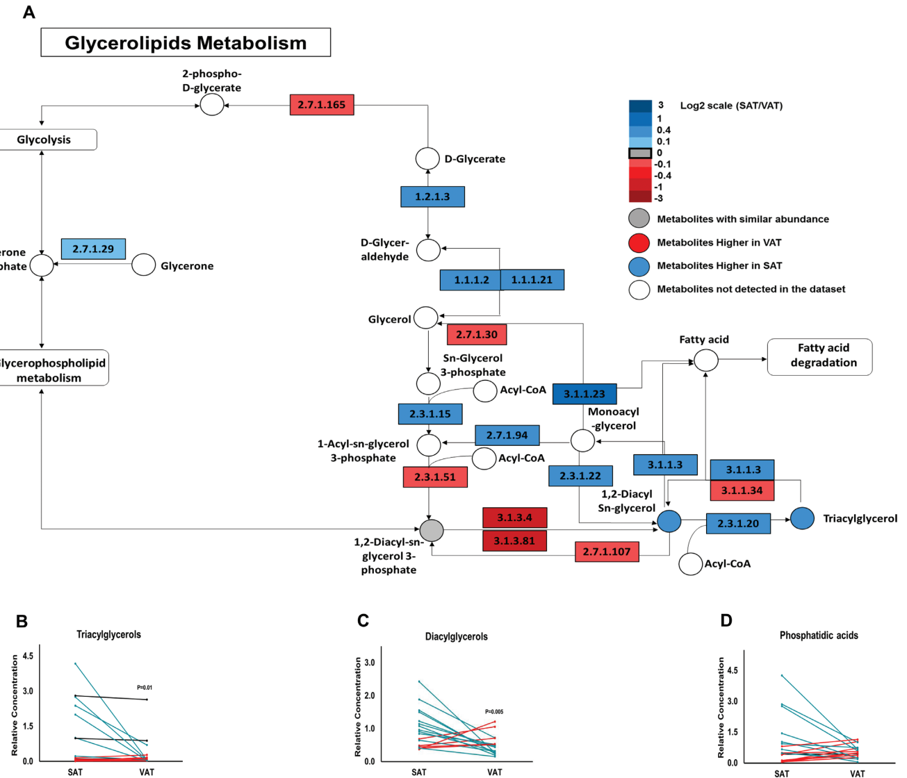
FIGURE 4 High levels of TAGs and DAGs found in SAT compared to VAT. (A) A metabolic map of the glycerolipid pathway (25). The gene expression of enzymes of the pathway as found in the GTEx database is shown as rectangles and the relative lipid accumulation found by our lipidomics study in the main data set is shown as circles. (B–D) The accumulation of glycerolipid groups found by our lipidomics study. Blue lines represent a change of \geq 10\% in the SAT:VAT ratio. Red lines represent a change of \leq -10\% in the SAT:VAT ratio. Black lines represent a similar accumulation \pm 10\% . n = 17 ; error bars represent SEMs; 1-tailed paired t test. DAG, diacylglycerol; KEGG, Kyoto Encyclopedia of Genes and Genomes; SAT, subcutaneous adipose tissue; TAG, triacylglycerol; VAT, visceral adipose tissue.
